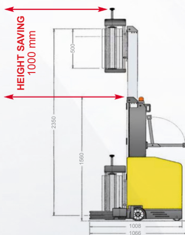
TELESCOPIC MAST
